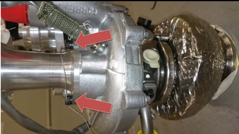
B) Restrictor Side
